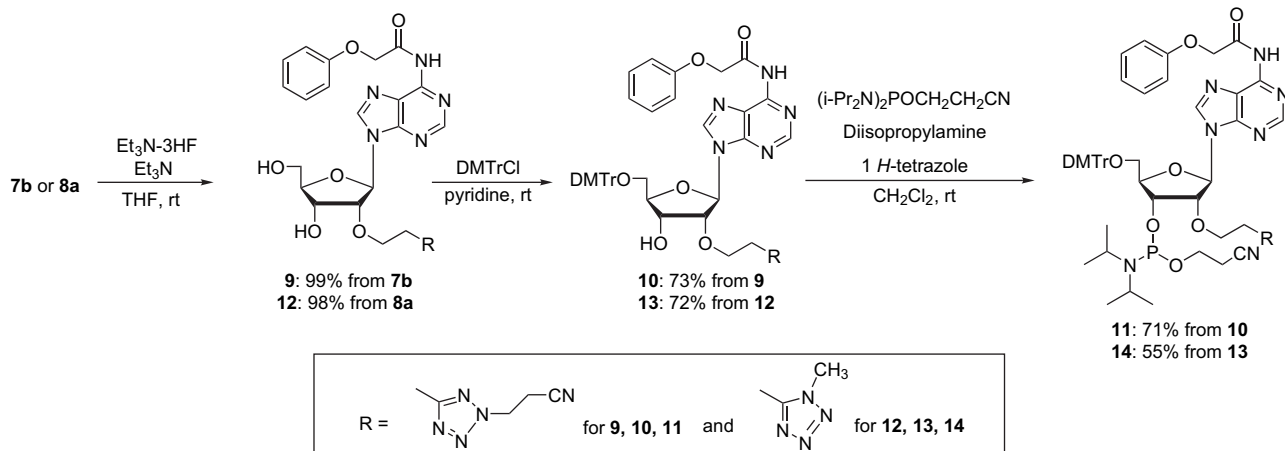
Scheme 2. Synthesis of protected adenosine 3'-phosphoramidite derivatives.
