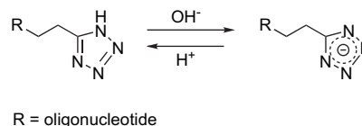
Figure 1. Interconversion between a neutral and a dissociated species of the tetrazole moiety.
