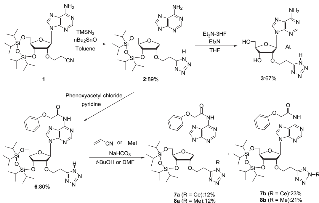
Scheme 1. Synthesis of 2'-O-[(1 H -tetrazol-5-yl)ethyl]adenosine derivatives and its N -alkylated derivatives.
